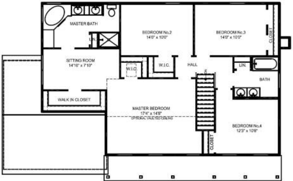
Second Floor Plan - 1,261 s/f
