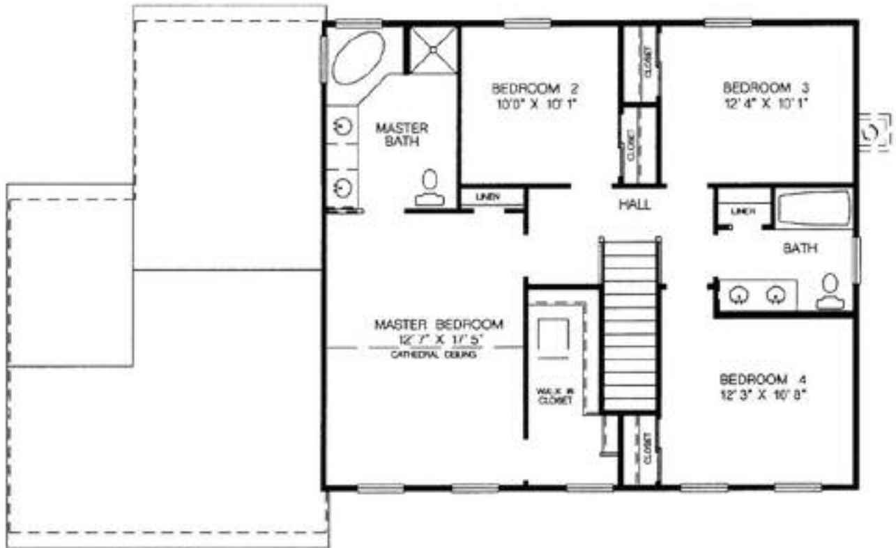
Second Floor Plan – 948 s/f
